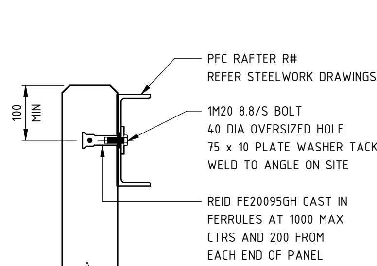
MARK FP2 PRECAST PANEL CLIP DETAIL
