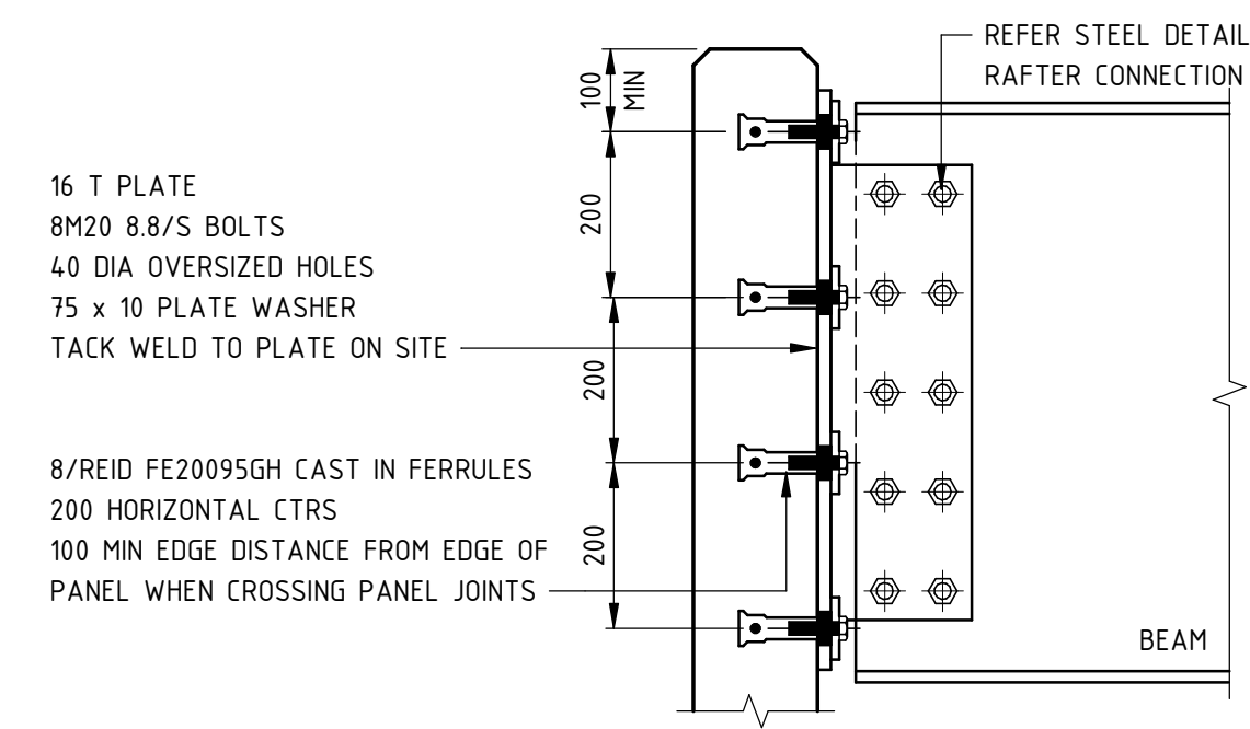
MARK FS6 PRECAST PANEL TO TRANSFER BEAM
