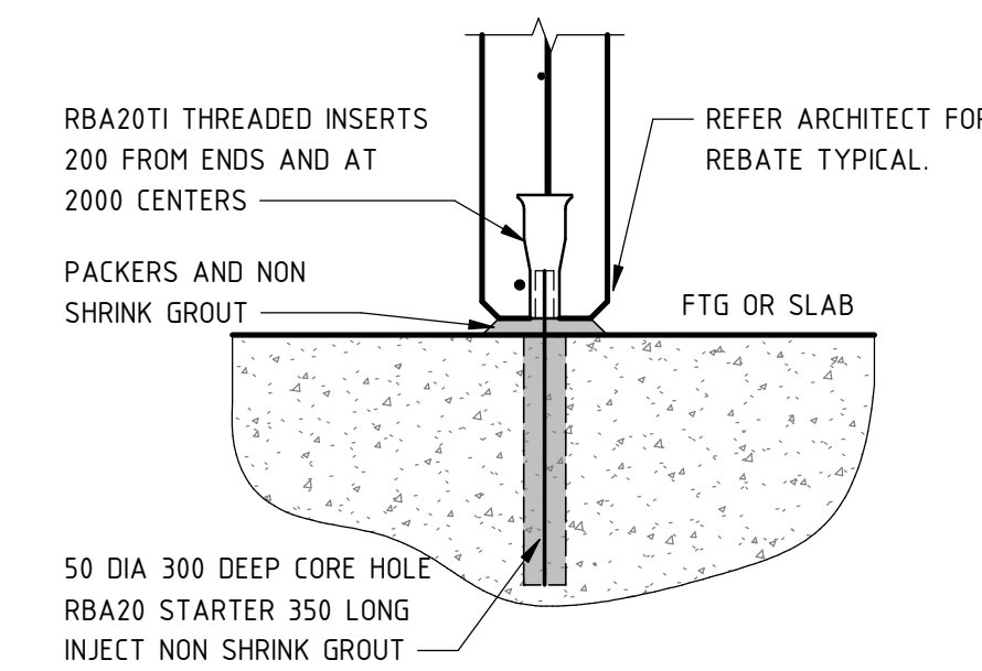
MARK FF1 PRECAST PANEL BASE DETAIL
