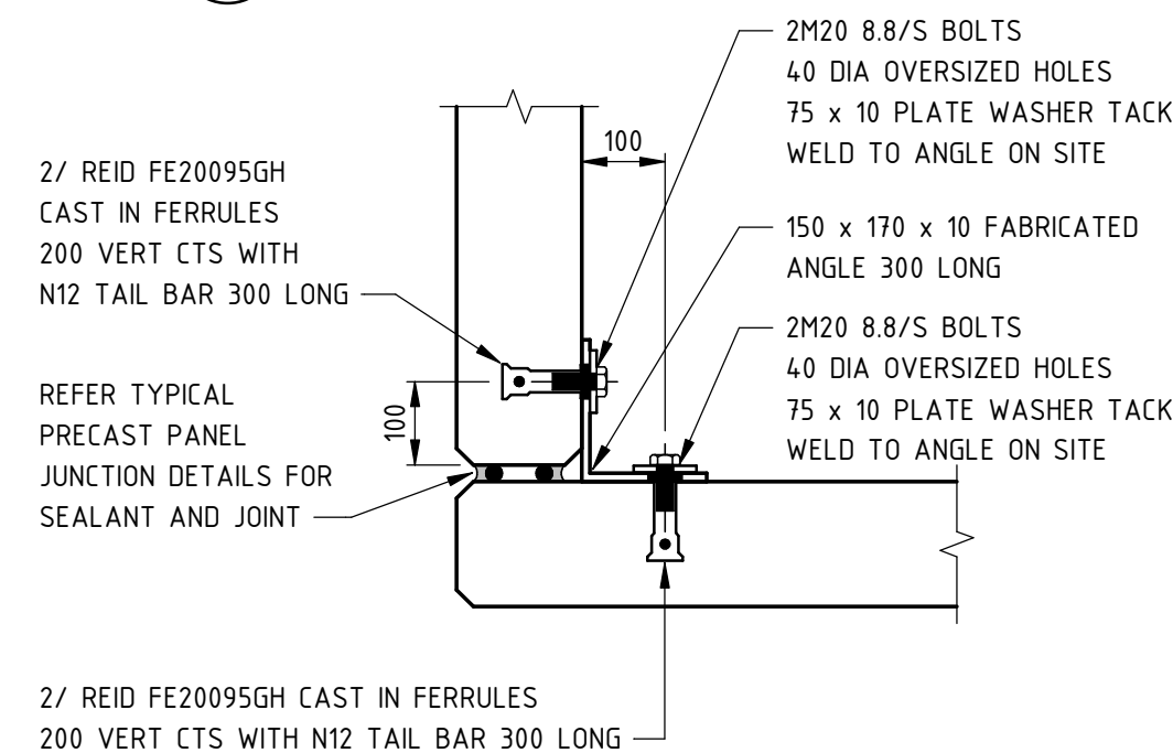
SECTION 2C SCALE 1 : 100
