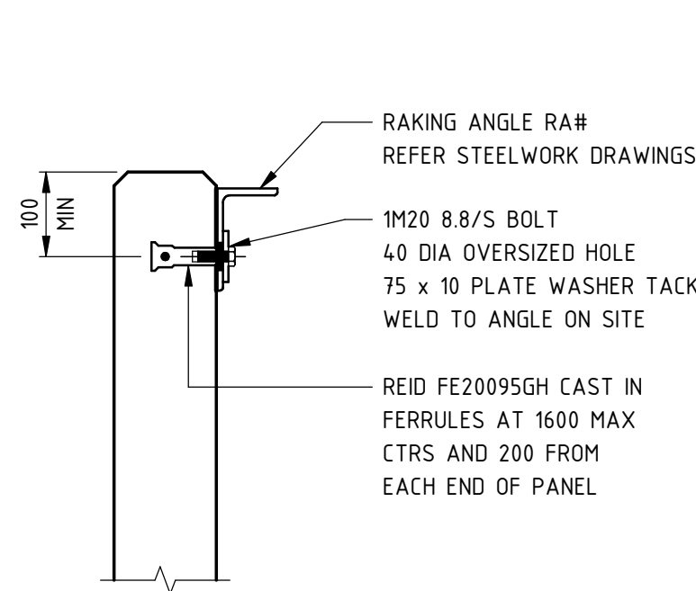
MARK FS2 PRECAST PANEL TO RAKING ANGLE CONNECTION
