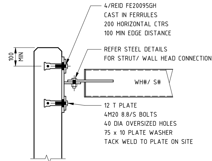
MARK FS3 STRUT/ WALL HEAD TO PRECAST PANEL
