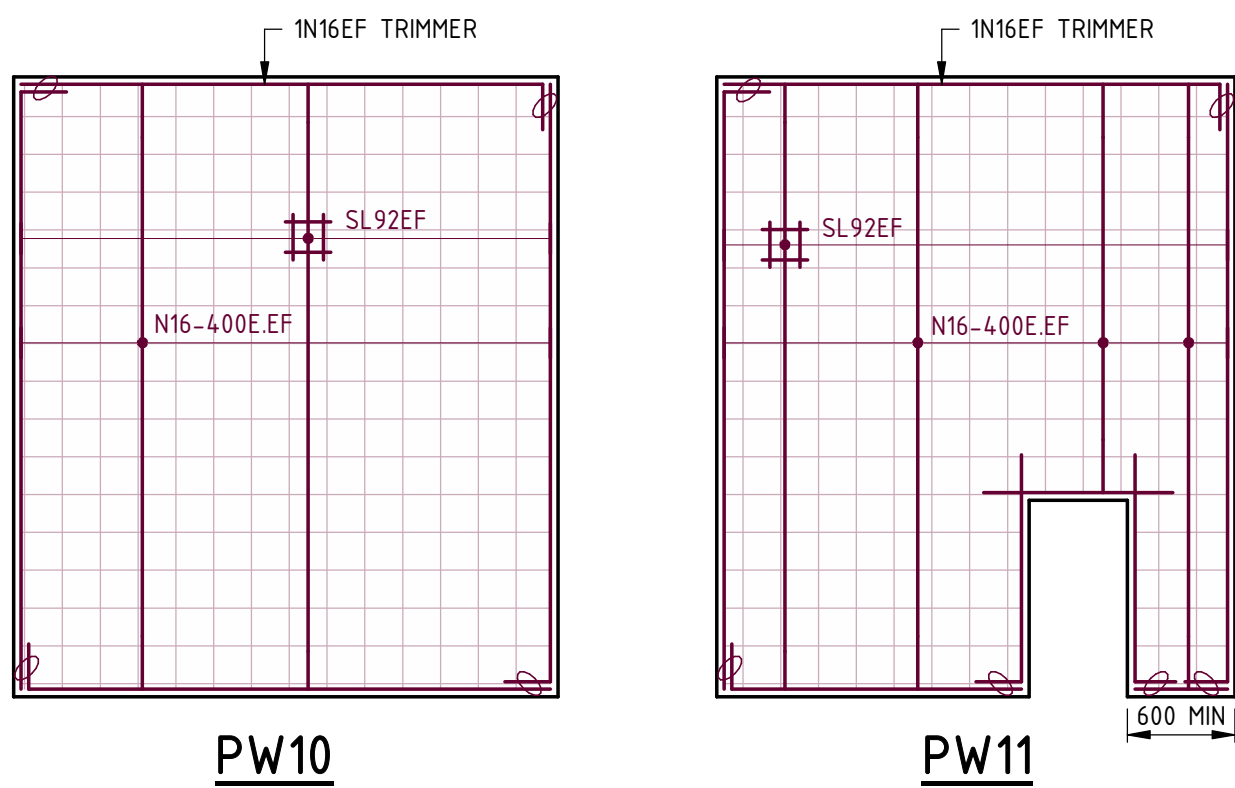
TYPICAL PRECAST TYPE DETAILS SCALE 1 : 100
