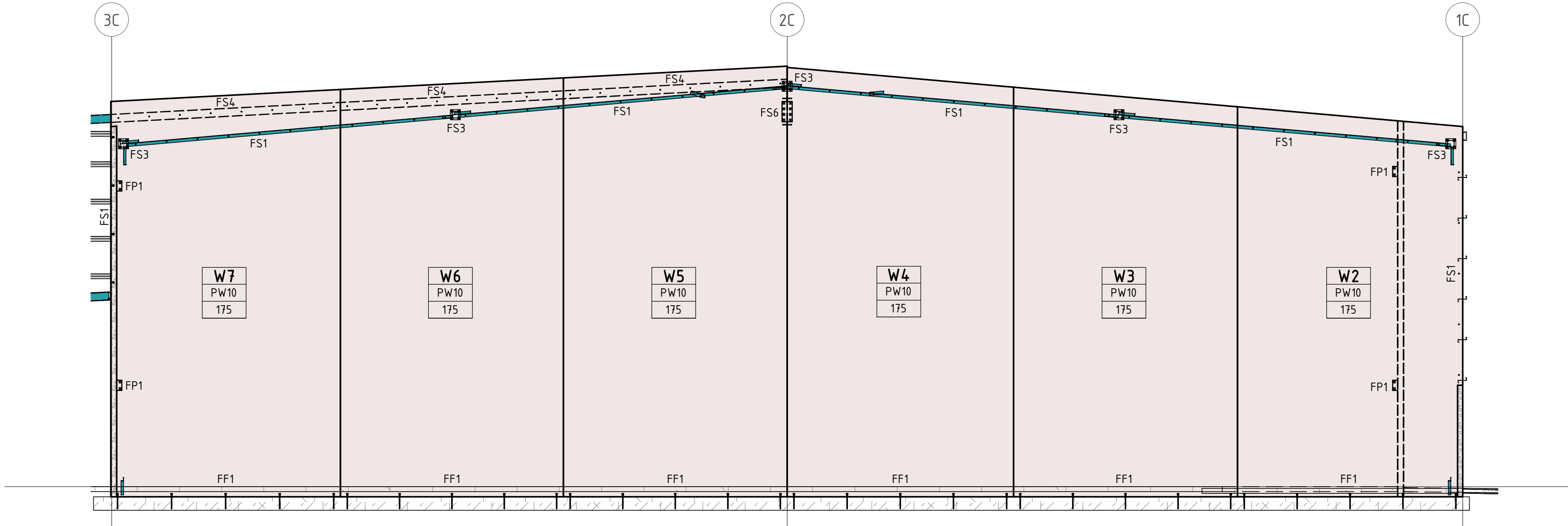
SECTION 2C SCALE 1 : 100
