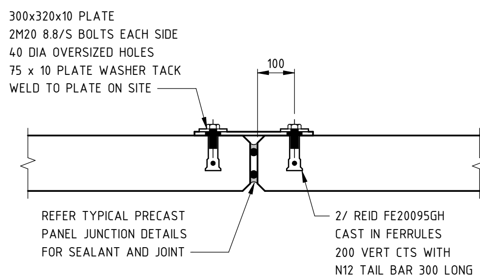
MARK FP2 PRECAST PANEL CLIP DETAIL
