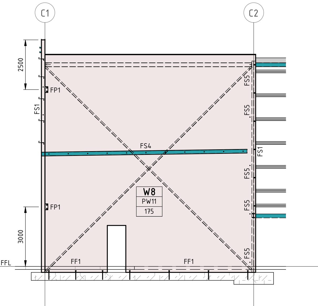
SECTION 3C SCALE 1 : 100
